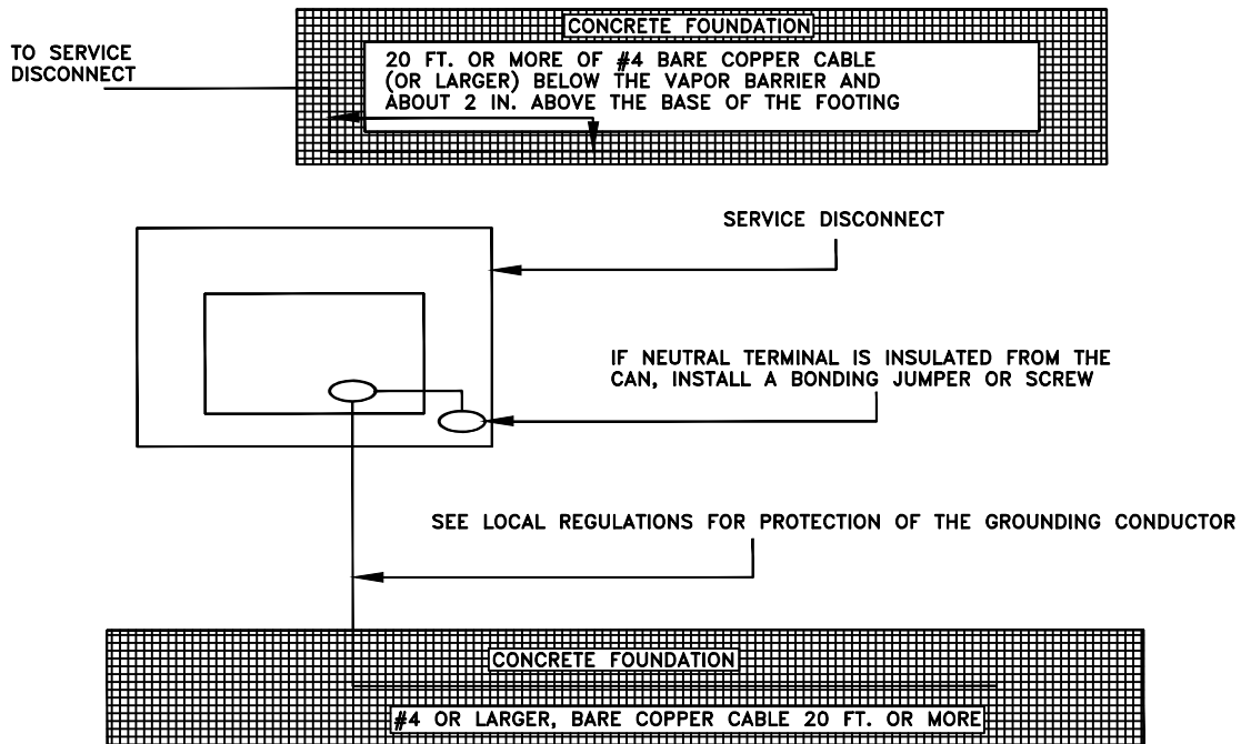
Figure 1 UFER Type Ground
