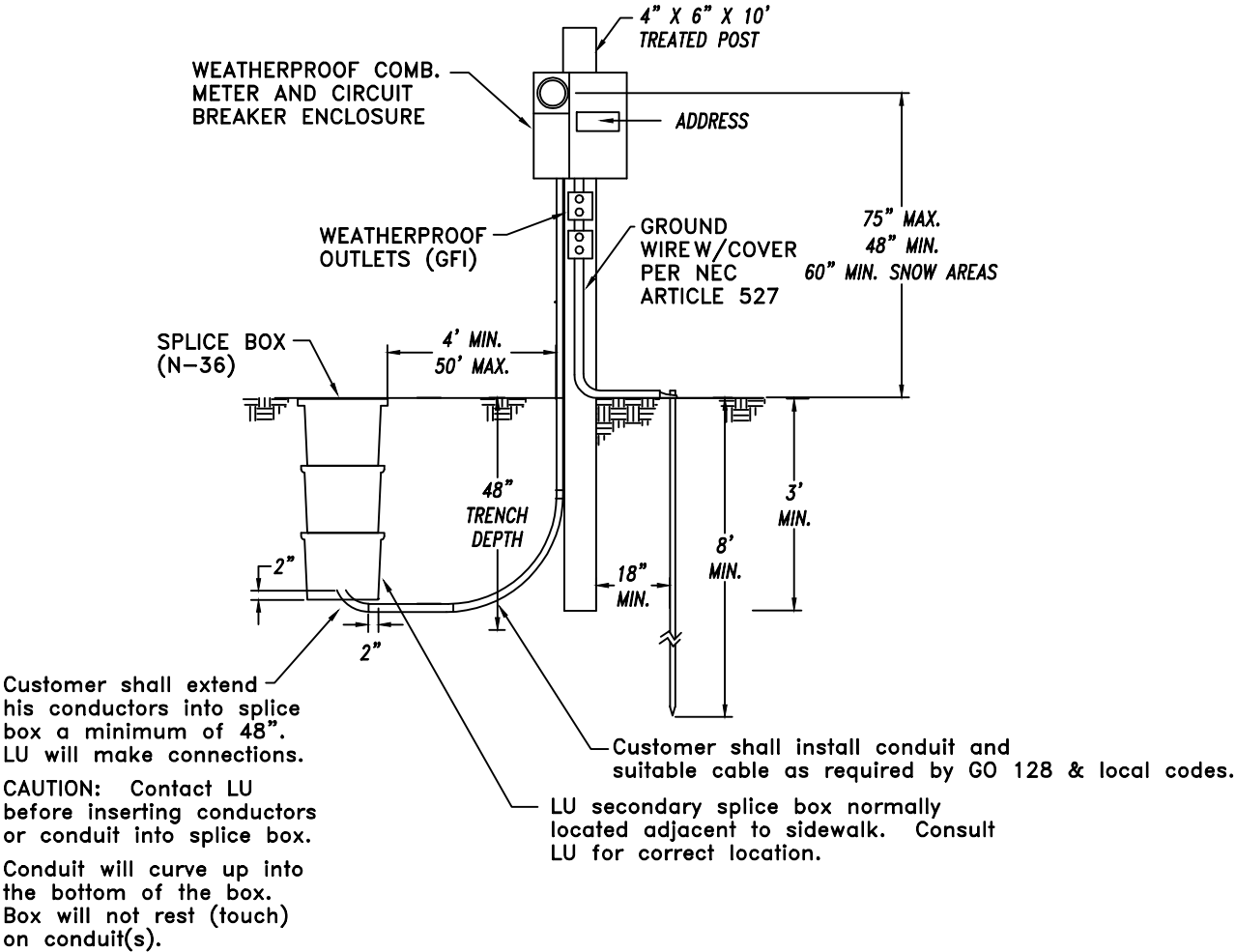
Total Temporary Service Detail
