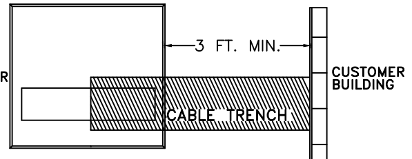
ALTERNATE #2 (TRANSFORMER SIDE ENTRY)
