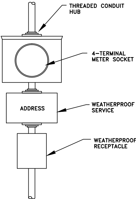
120/240V 3-WIRE WITH WEATHERPROOF SERVICE SWITCH AND RECEPTACLES.
