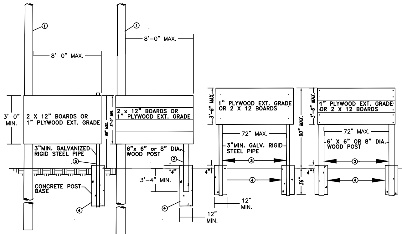
ALTERNATE PANEL BOARD CONSTRUCTION USING WOOD
