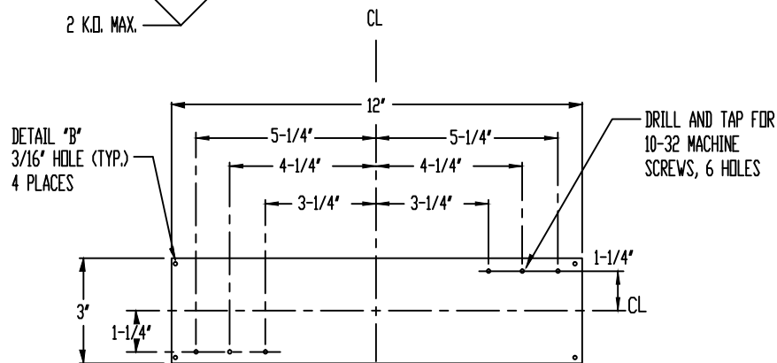
DETAIL "A" REMOVABLE TEST BLOCK PERCH
