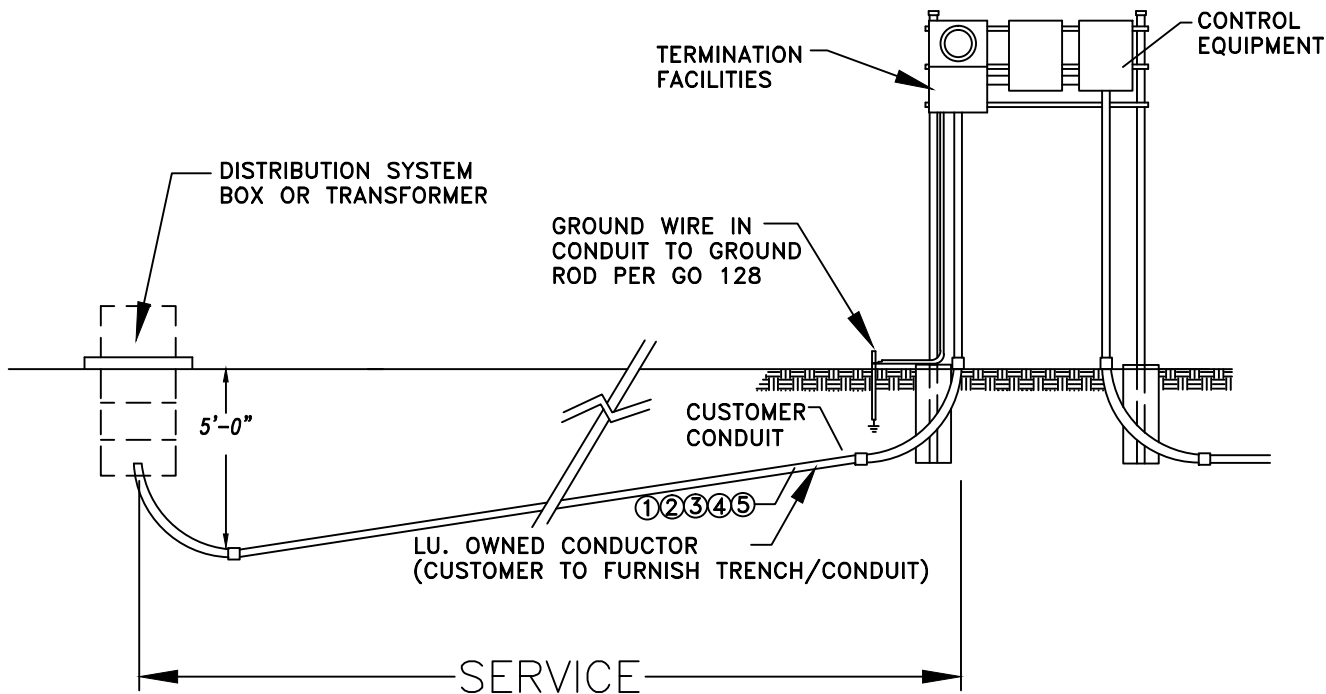
TYPICAL UNDERGROUND SERVICE USING PANEL
