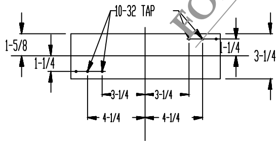
REMOVABLE TEST SWITCH MOUNTING BASE DETAIL
