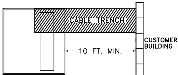
ALTERNATE #1 (TRANSFORMER FRONT ENTRY)
