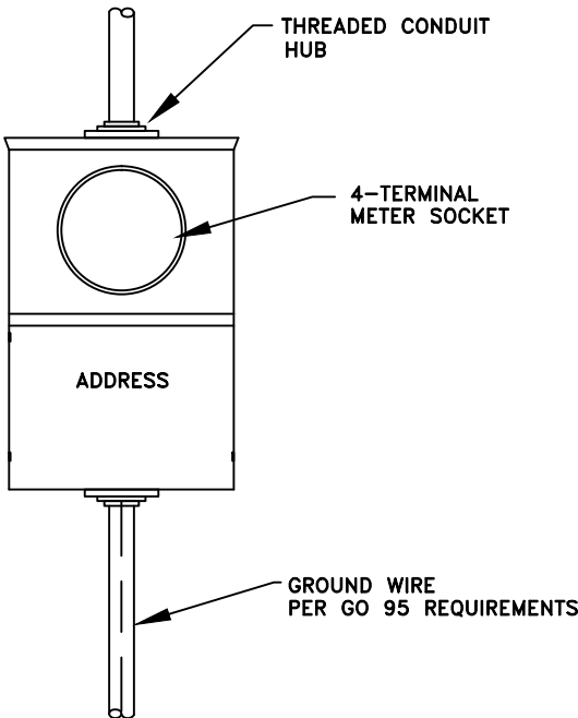
120/240V 3-WIRE WITH WATT HOUR METER, SERVICE SWITCH AND RECEPTACLE IN WEATHERPROOF CABINET.
