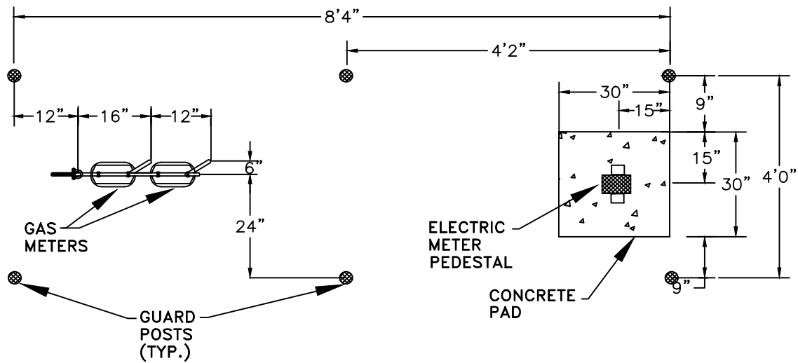
DETAIL #6C DUAL METERS
