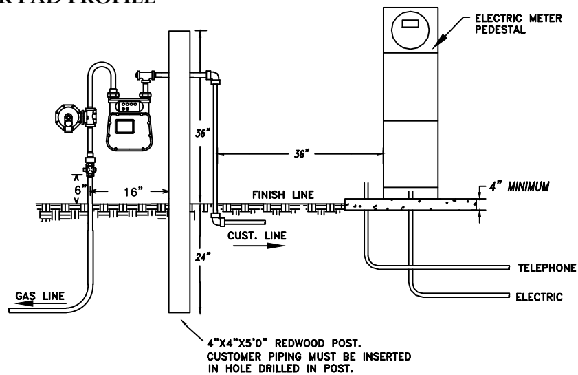
DETAIL #6A METER PAD PROFILE
